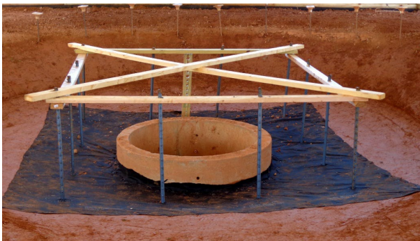
Figure IP-1 Silt Fence Inlet Protection installation showing geotextile underlayment, steel T-posts, 2 x 4 bracing, and dewatering device.
