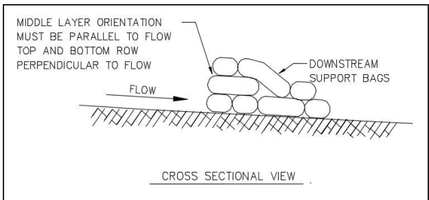
Figure CD-8 Sand Bag Check Dam Cross-Section
