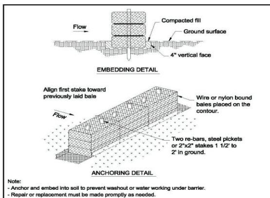
Figure ST-1 Placement of Straw Bales
