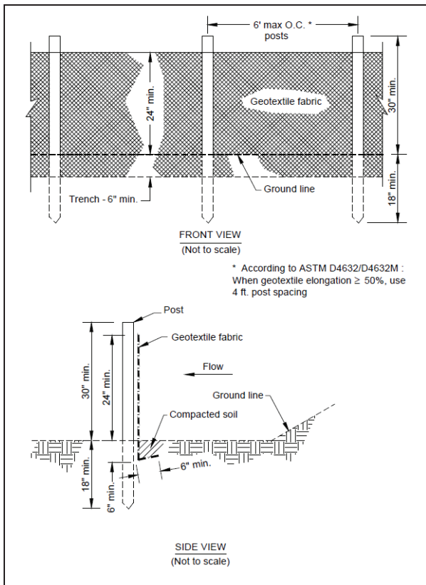
Figure SB-2 Detail of Type B Silt Fence
