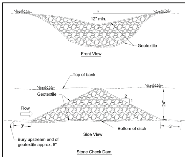
Figure CD-1 Views of a Typical Rock Check Dam
