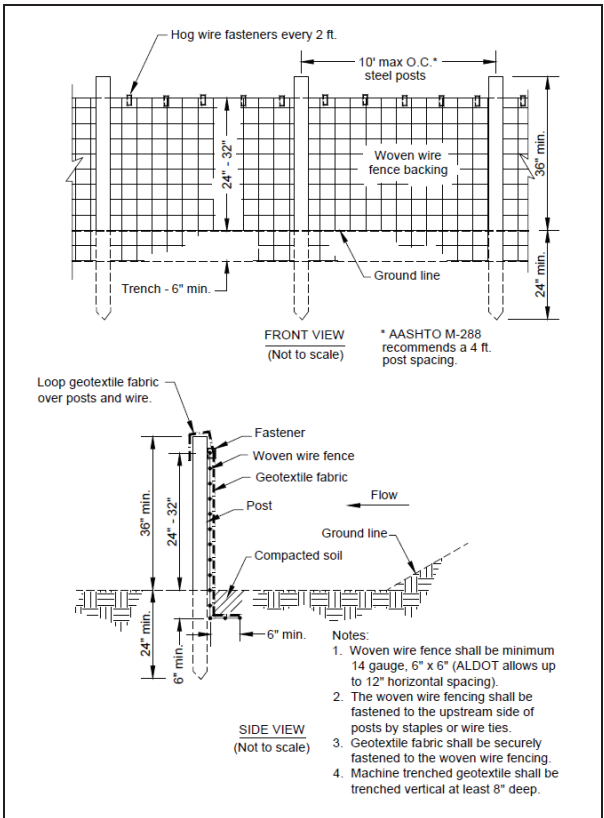
Figure SB-1 Detail of Type A Silt Fence
