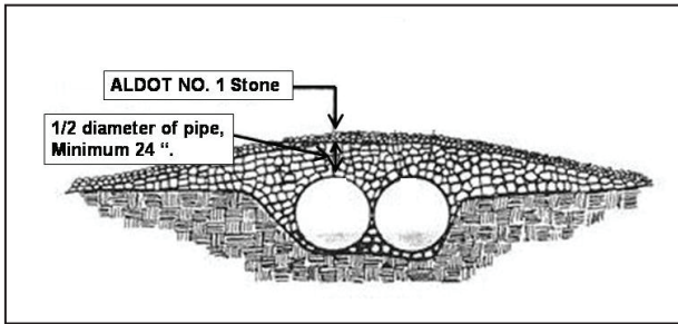
Figure TSC-2 Culvert Stream Crossing
