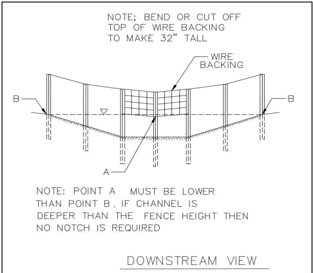
Figure CD-5 Silt Fence Check Dam Cross-Section
