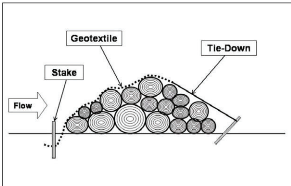
Figure BFB-1 Brush/Fabric Barrier
