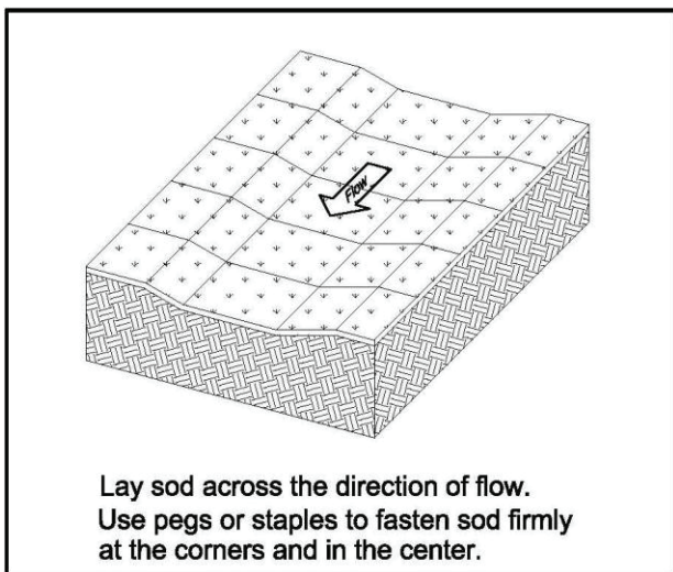
Figure SOD-2 Installation of Sod in Waterways
