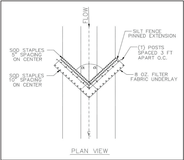
Figure CD-6 Silt Fence Check Dam Plan View
