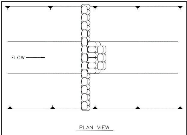
Figure CD-9 Sand Bag Check Dam Plan View
